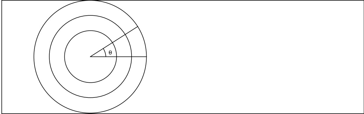
Figure 4. Arc Length Problem
