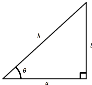
Figure 2. A standard right triangle trigonometry diagram
